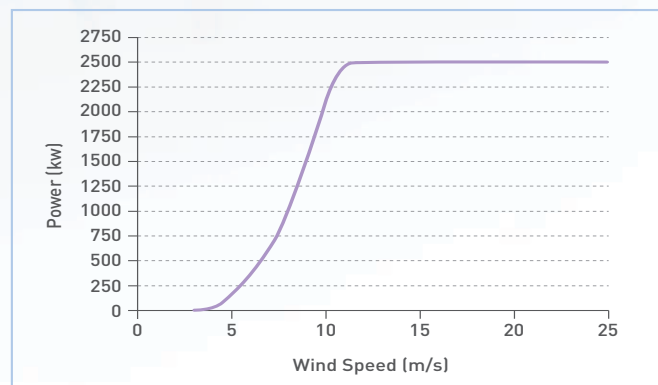
| AV928 Power Curve |
